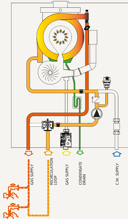
RECIRCULATION MODE (POST CIRCULATION): RECIRCULATION ACTIVE
